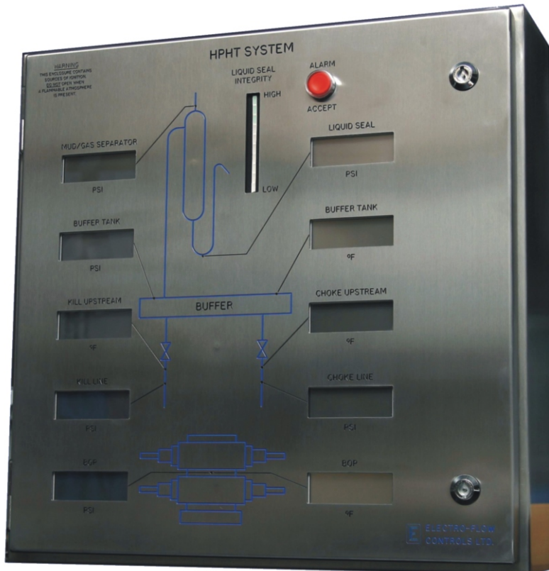
Temperature & Pressure displays with Liquid Seal Monitor
